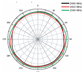
Horizontal (H Plane)
